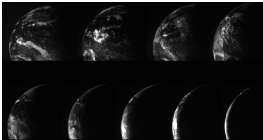
SMART-1's view of a waning Earth These pictures were taken with the AMIE camera on board SMART-1 on 1 and 2 November 2004 when SMART-1 was on course for its last close approach to Earth, before being captured by the Moon's gravity in mid-November.
