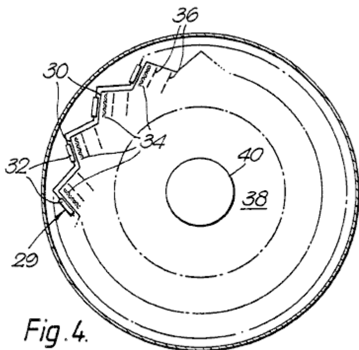
Fig. 4 is a diagrammatic section through one form of converter using electrons, showing a circular series of electron sources;
