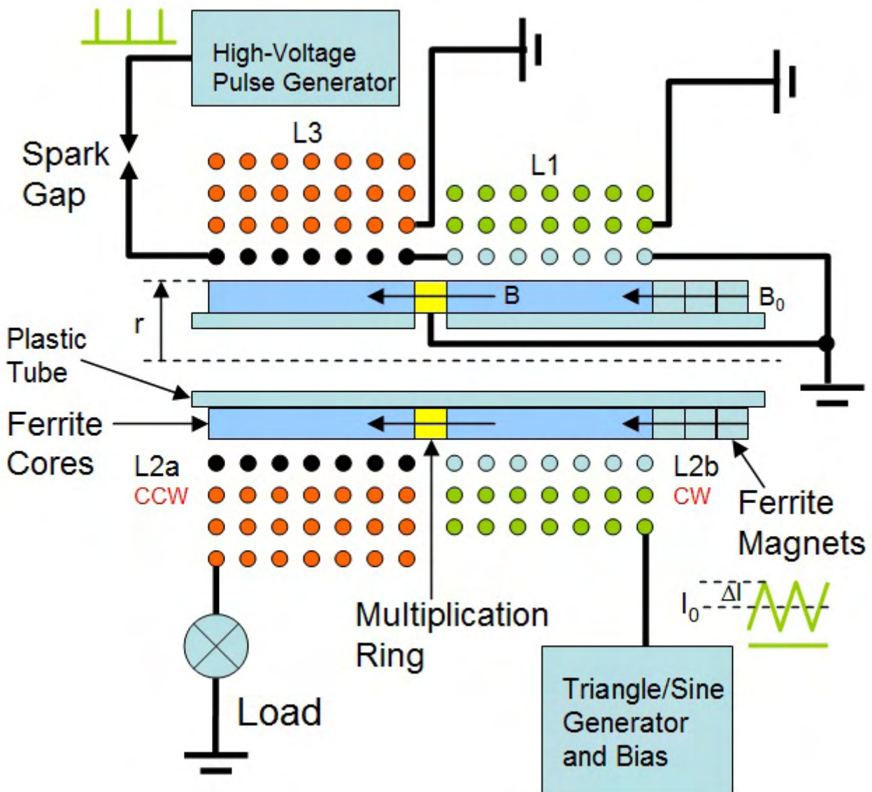
Fig.5 Cross-section of the Kapanadze-like energy device. Some of the actual implementation details may differ from the arrangement shown above, but that will not alter the operation of device. This diagram is not to scale.
