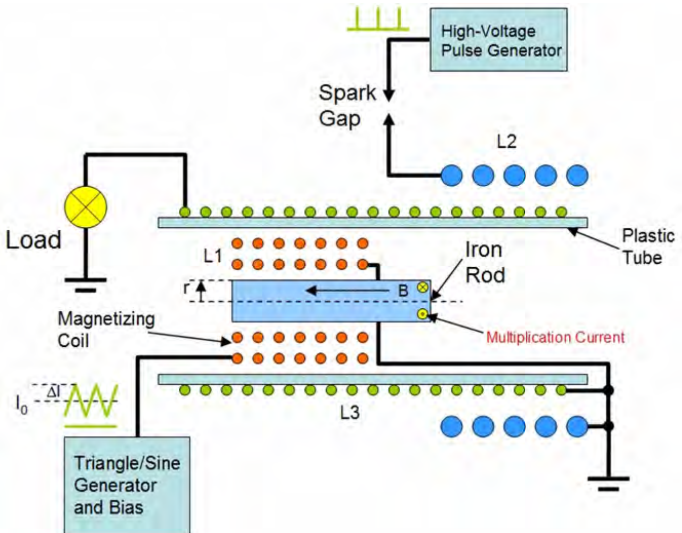
Fig.4 Iron rod based example coil. In reality, coil L1 may have hundreds of turns. The arrangement of the coils is different in various implementations of the device. This drawing is not to scale.
