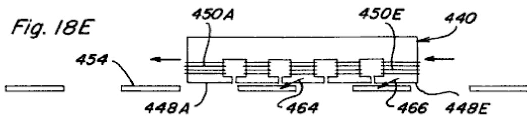
Figs.18A-18E show a linear motion device;
