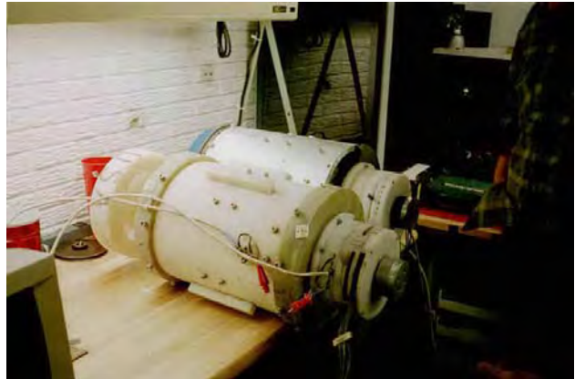
EMA4 and EMA5 Motors as Found in 2000
