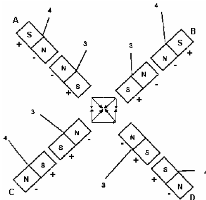
Fig.11 - is an electromagnetic diagram representation of north and south poles of the sets of coils (A, B, C and D).
