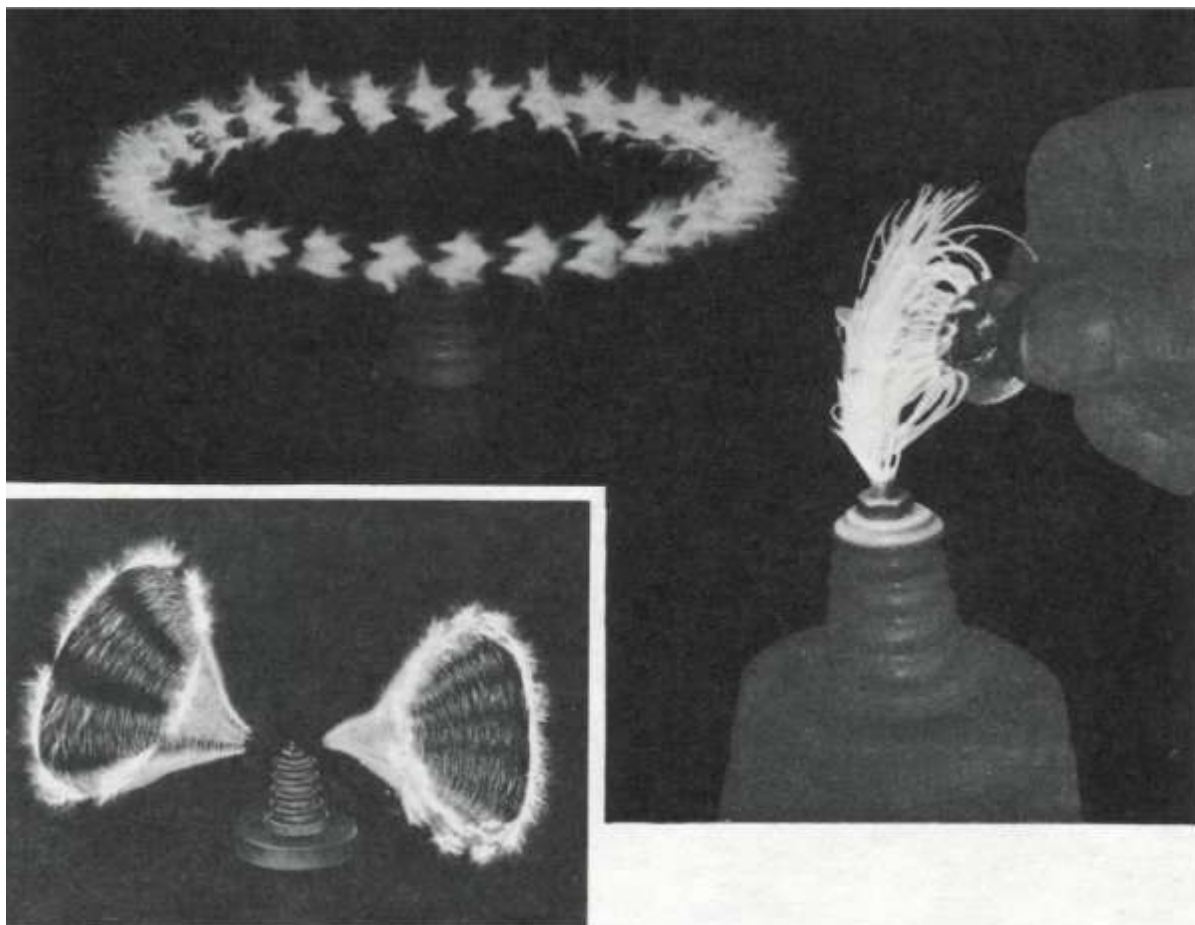
Spectacular fireworks include a ring of fire scribed by a wire pivoting on a phonograph needle attached to a terminal. A finer wire, attached directly to a coil, produces trumpet pinwheels, shown in the smaller photo. This article tells how you can create these fireworks
