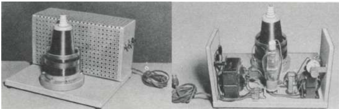
Neat housing presents a coil on a platform with all the wiring running underneath to the transformer section behind the perforated metal cover. Note the switches on the right side of the housing
